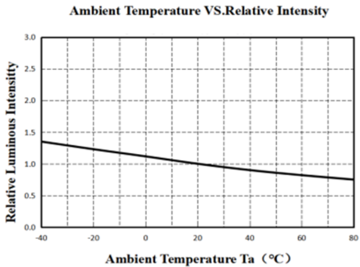
Fig 6. Temp.v/s Lumens current
