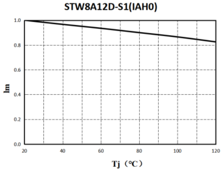
Fig 7. Junction Temperature vs. Relative Luminous Intensity, I_F=60\text{mA}
