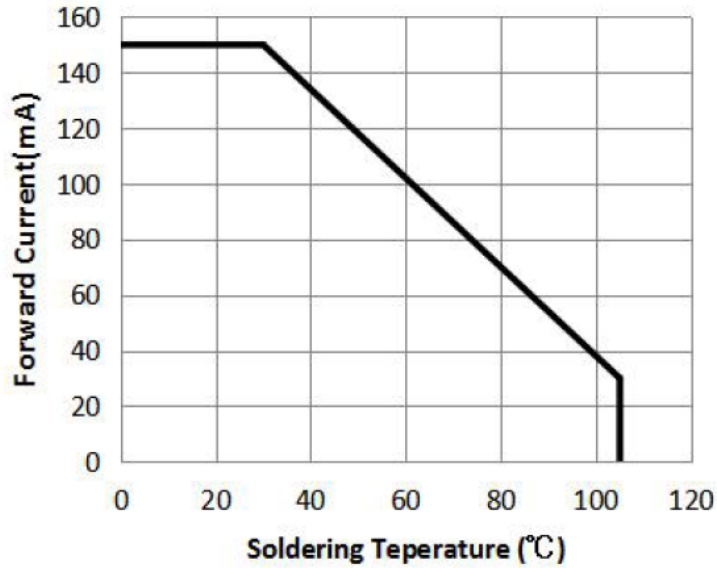
Fig 5. Solder Temp.v/s Forward current (Derating curve)
